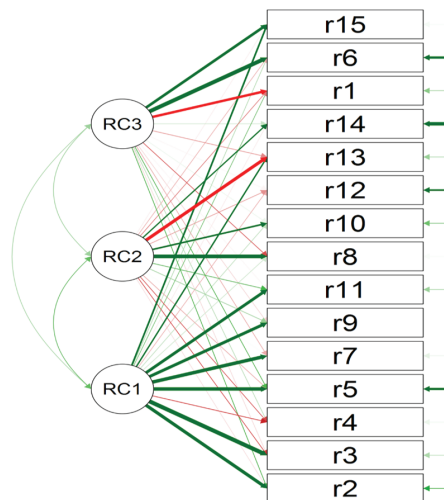
Fig 2. Path Diagram
